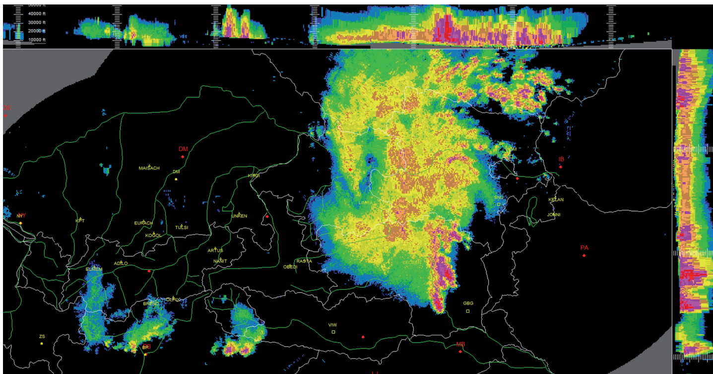
Weather radar
